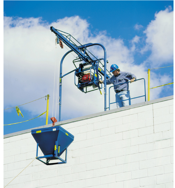
TT1000 Trolley Hoist w/ GB800 Gravel Bucket
